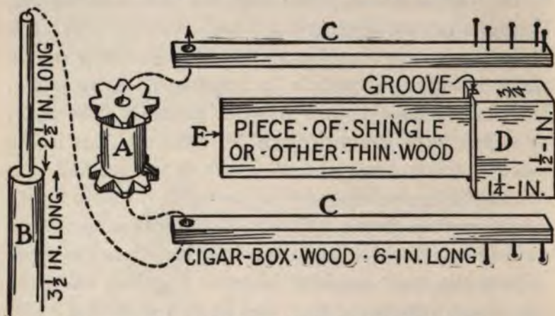
FIG. 116. — Details of the Noisy Cricket-Rattle shown Fig. 114.
